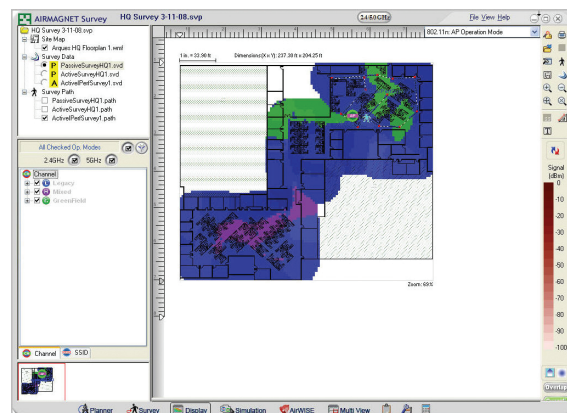
Figure 5: 802.11n Operation Mode coverage map
