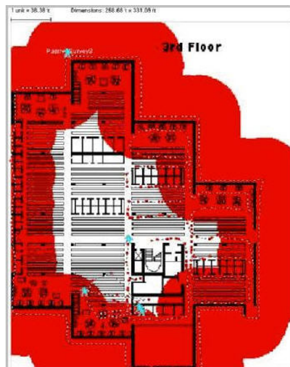
Figure 4: RF spillage outside the corporate building
