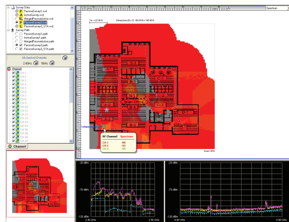
Figure 7: Wi-Fi and non Wi-Fi data in a single survey
