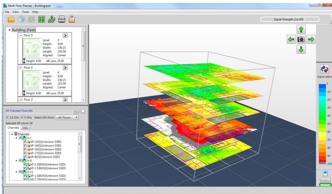
Figure 10: Automated WLAN modeling using AirMagnet Planner
