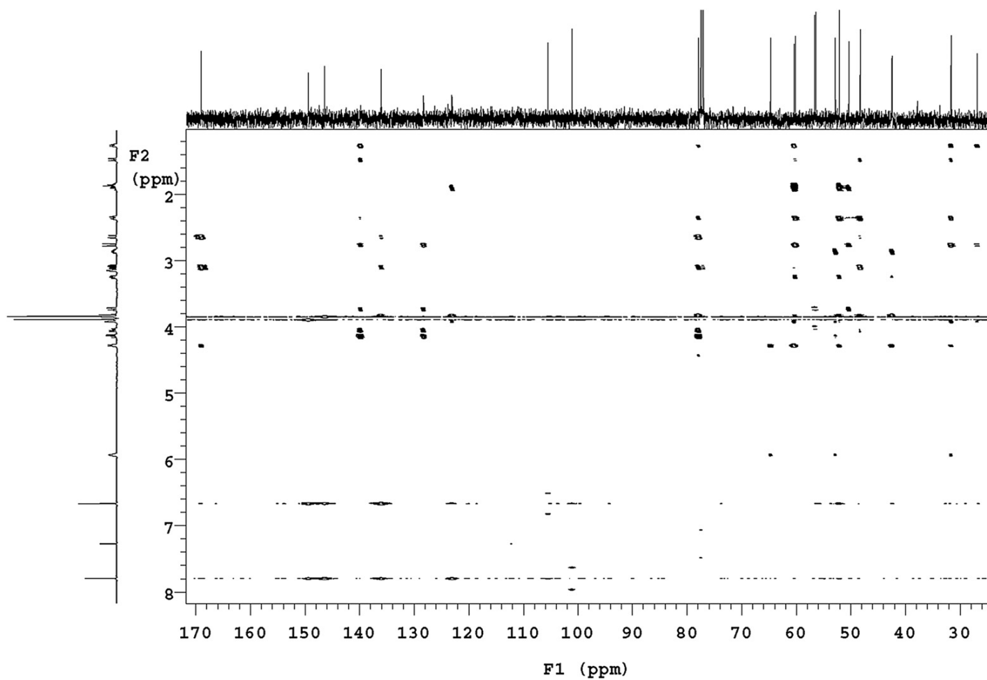
Figure 15.6.gHmbc: The 2-D ^1\text{H} - ^{13}\text{C} gHMBC NMR spectrum of brucine in \text{CDCl}_3 .
