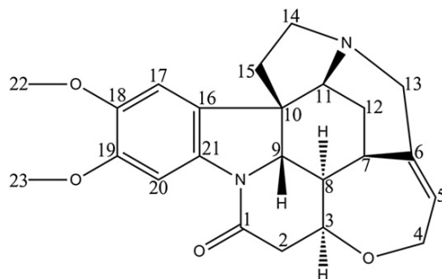
Figure 15.6.struc: The structure of brucine (with numbering).
