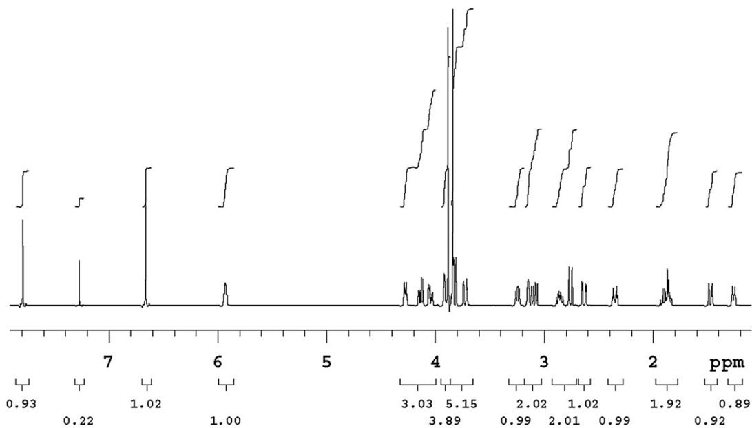
Figure 15.6.h: The 1-D ^1\text{H} NMR spectrum of brucine in \text{CDCl}_3 .
