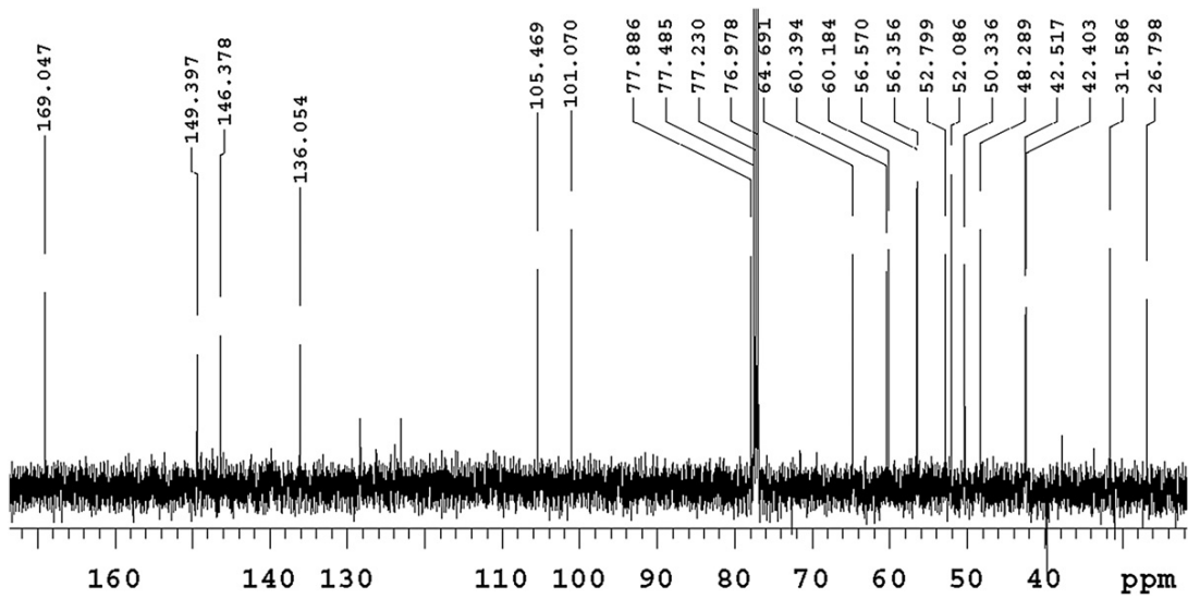
Figure 15.6.c: The 1-D ^{13}\text{C} NMR spectrum of brucine in \text{CDCl}_3 .
