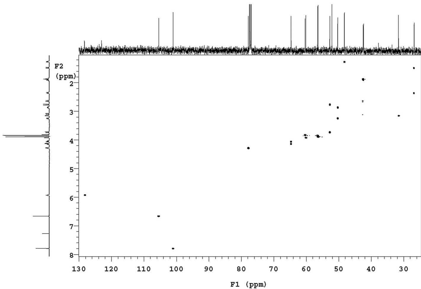
Figure 15.6.hsqc: The 2-D ^1\text{H} - ^{13}\text{C} HSQC NMR spectrum of brucine in \text{CDCl}_3 .
