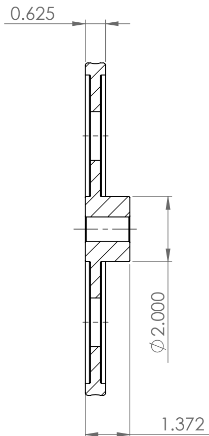
SIDE (BREAKOUT)
