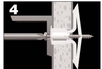
4 Place item over anchor. Insert screw and tighten until flush with item—then stop. Do not overtighten.
