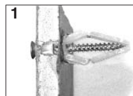
1 Short screw in competitive anchor—misses apex; NO holding power
