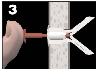
3 Insert key to pop anchor open behind hollow wall (not necessary for thick or solid walls). Do not hammer key. Remove. key.
