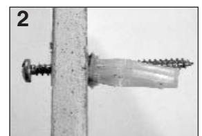
2 Screw at angle in competitive anchor—misses apex; NO holding power
