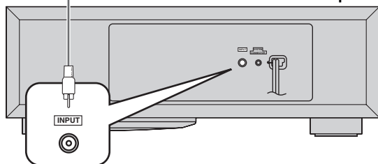
YST-FSW050 rear panel
