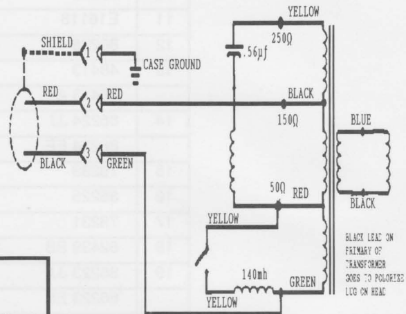
WIRING DIAGRAM
