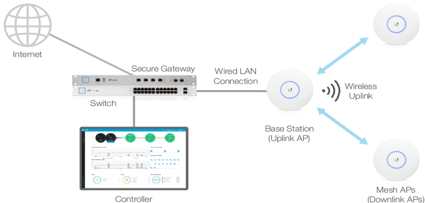
Example of Wireless Uplink Topology with UAP-AC-PRO
