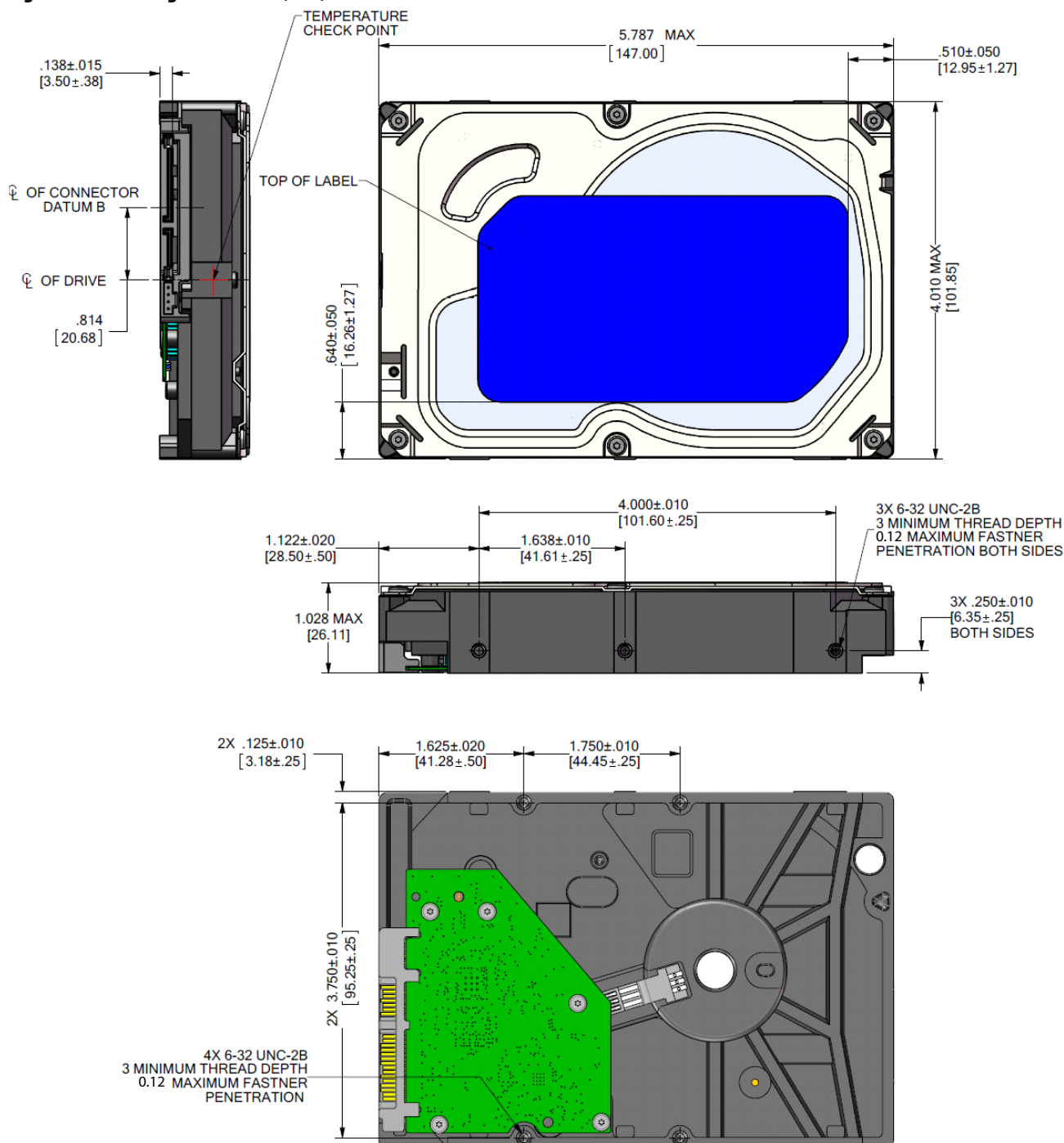
Figure 2 Mounting dimensions (4TB)
