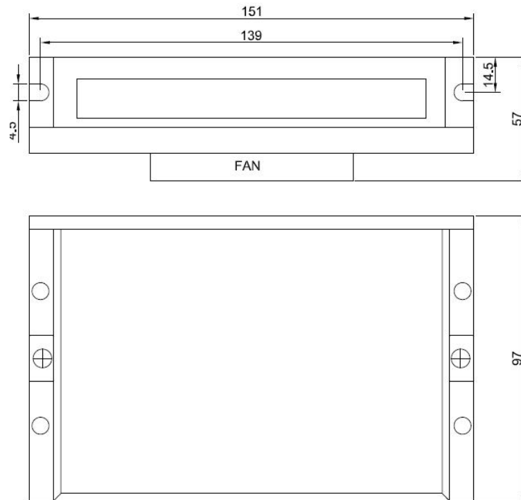
Figure 1: Mechanical specifications
