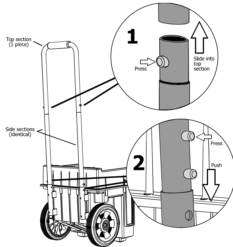
Figure 2 - Handle Assembly
