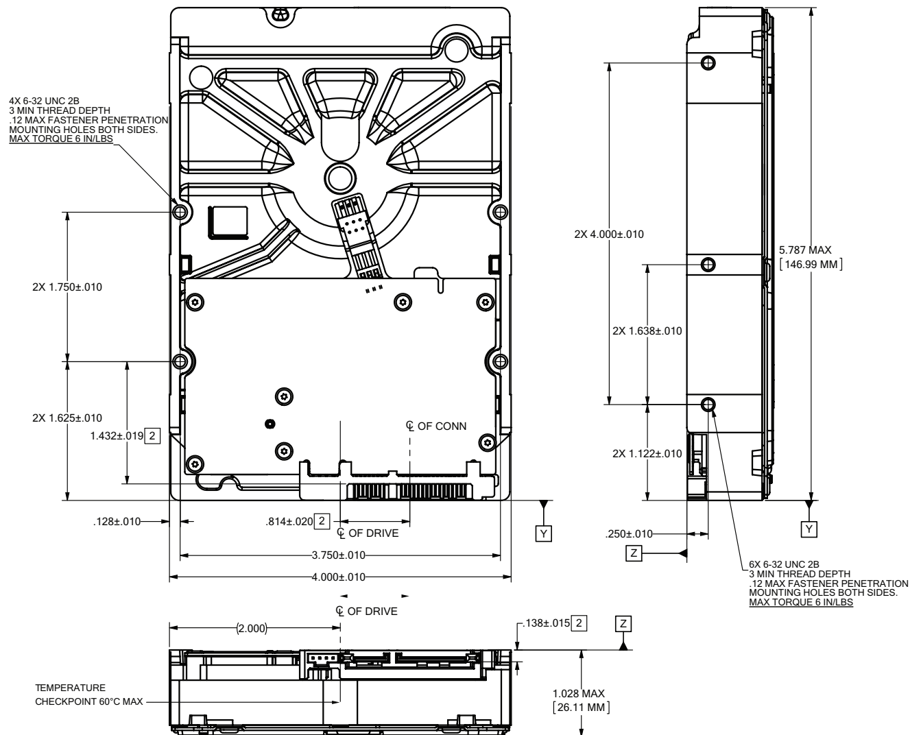
Figure 4 Mounting dimensions (6TB)
