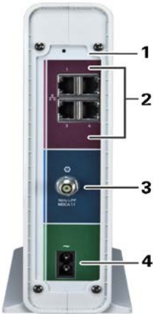
Figure 2 – SBG6782-AC Rear View
