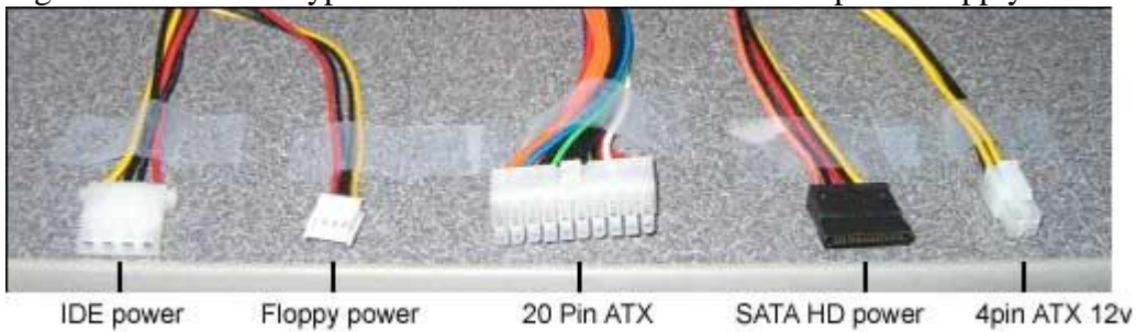
Figure below shows typical cable connection found on the power supply
