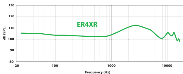
ER4XR Frequency Response
