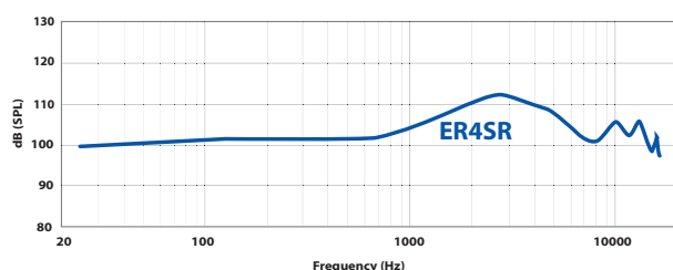
ER4SR Frequency Response
