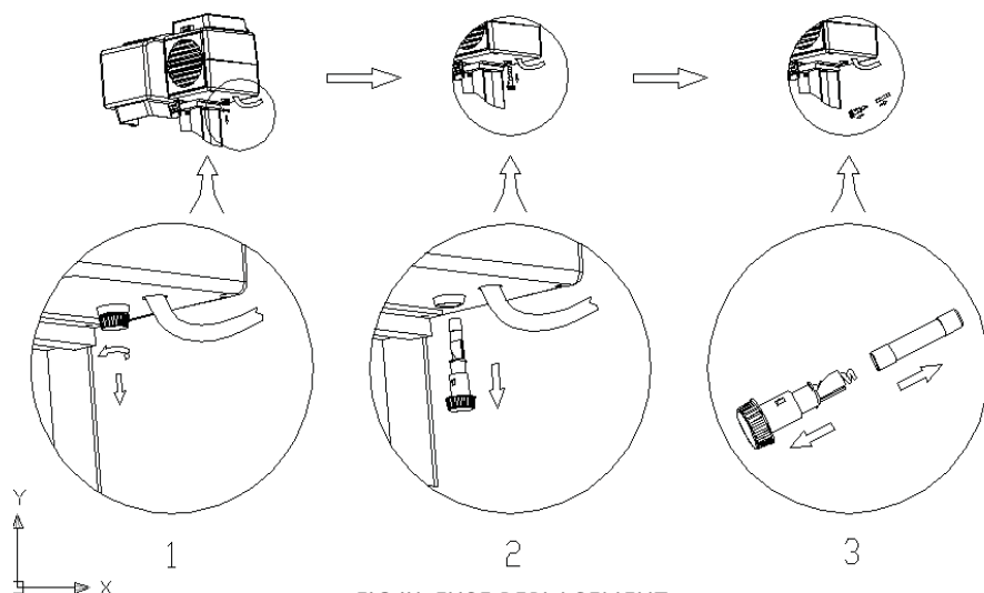
FIG IX: FUSE REPLACEMENT
