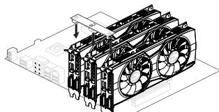
3-way SLI: Install the third GeForce card into the tertiary PCI Express slot on the motherboard. Connect the GeForce cards together using the 3-way SLI bridge connector that came with your SLI-ready motherboard.
