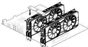
2-way SLI: Install your second GeForce graphics card in to the secondary PCI Express x16 slot. Connect the two cards together using the 2-way SLI bridge connector that came with your SLI-ready motherboard.
