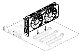
Install your first GeForce graphics card into the Primary PCI Express x16 slot.
