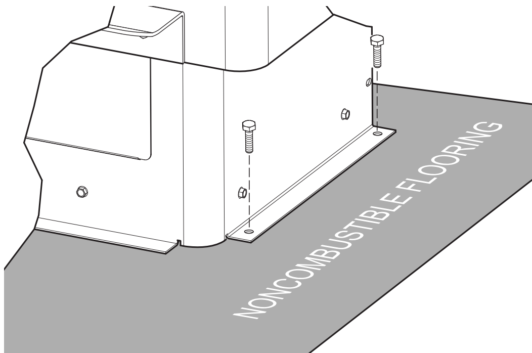
Illustration: Securing heater to the Floor.
