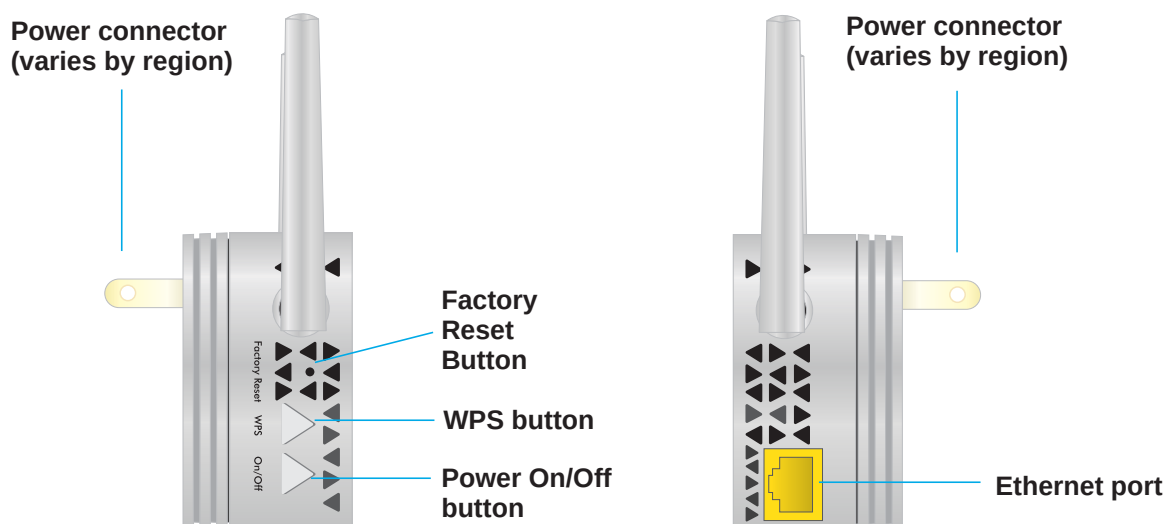
Figure 2. Side panel buttons and port
