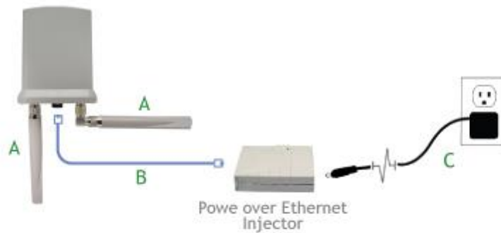
Hi-Gain™ Outdoor Wireless-N Dual Radio Smart Repeater
