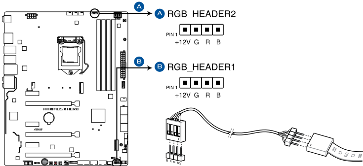
ROG MAXIMUS X HERO RGB_HEADER connectors
