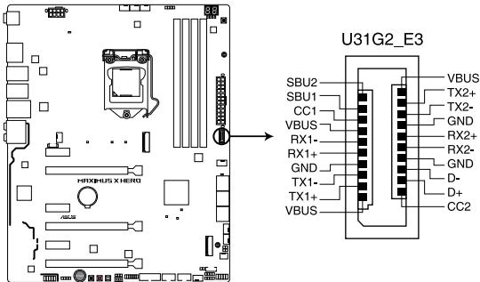
ROG MAXIMUS X HERO USB 3.1 Gen 2 front panel connector
