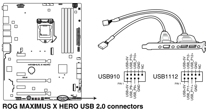
ROG MAXIMUS X HERO USB 2.0 connectors
