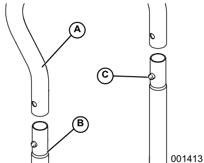
Figure 2-1. Insert Handle
