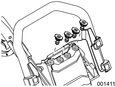
Figure 2-3. Insert Nozzles
