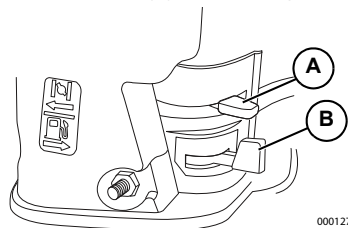
Figure 3-2. Fuel Valve and Choke
