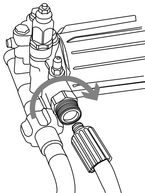
Figure 2-11. Connect High-Pressure Hose to Pump
