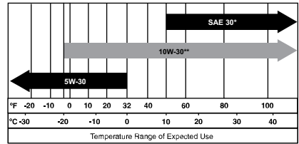
Figure 4-4. Oil Viscosity
