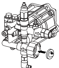
Figure 2-8. Inspect Inlet Screen
