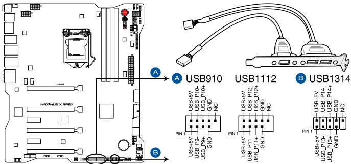
ROG MAXIMUS X APEX USB 2.0 connectors
