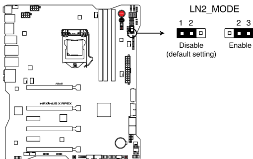
ROG MAXIMUS X APEX LN2 Mode jumper
