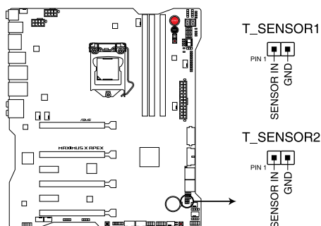
ROG MAXIMUS X APEX T_SENSOR connectors
