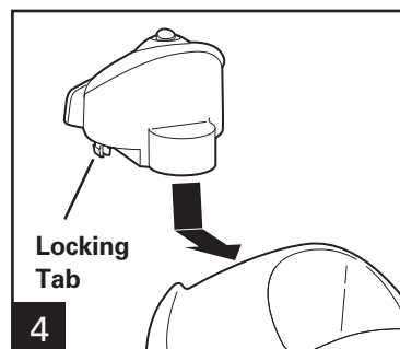
To assemble lid and motor housing, align the two locking tabs on motor housing with openings on lid. Snap into place.
