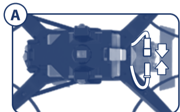
Connect battery plugs on the underside of the racer to turn it on.
