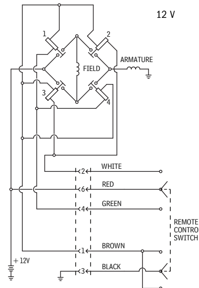
ELECTRICAL CIRCUIT DIAGRAMS
