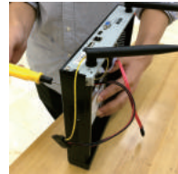
Insert the hard drive, secure it to the bottom of the unit with the four screws
