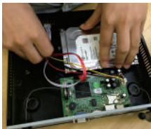
Connect the data wire and power wire as shown
