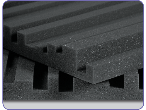
Studiofoam® Metro™ - Overall NRC 0.70*
