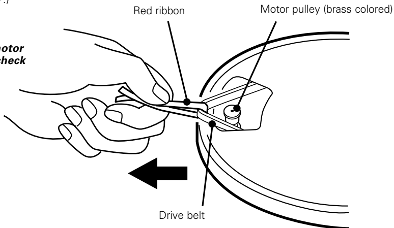
Figure 2 – Assembling the turntable
