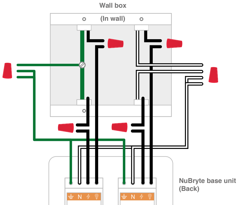
Typical Double Gang Wiring
