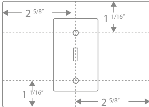
Required clearance to replace existing single gang toggle and round switch
