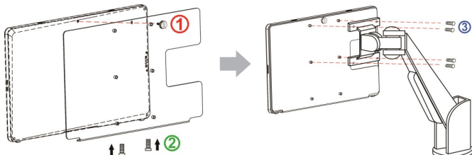
Fig: ①②Screw Multi-Mount Kit to On-Lap monitor and ③screw monitor with Multi-Mount Kit to VESA 100 arm.
