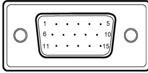
15-Pin Color Display Signal Cable
