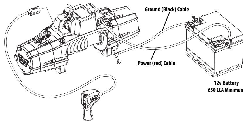
Figure 4 Electrical Diagram
