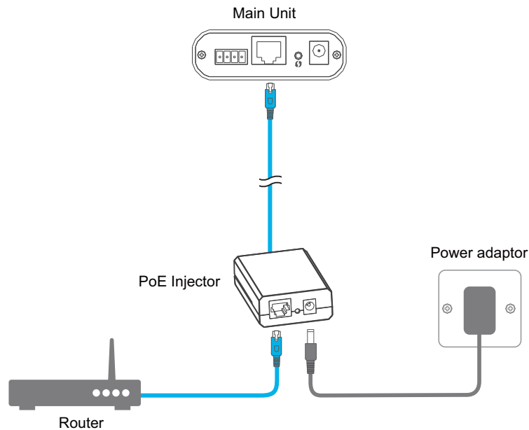
PoE injector connection diagram
