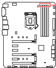
DIMM LEDs
