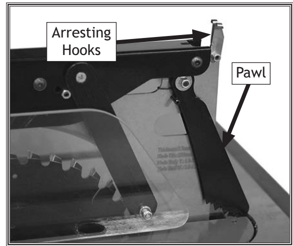
Figure 47. Pawls in return position.
