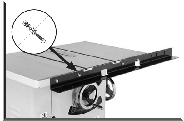
Figure 16. Front rail installed (W1819).
