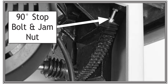
Figure 94. 90° stop bolt and jam nut.
