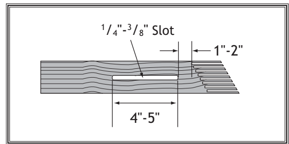
Figure 71. Slot routed in featherboard.
