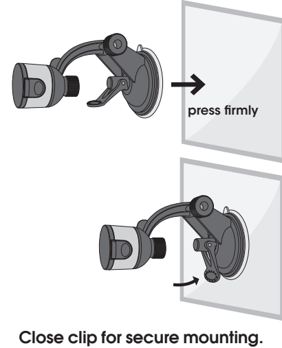
3 Dashboard Mount
