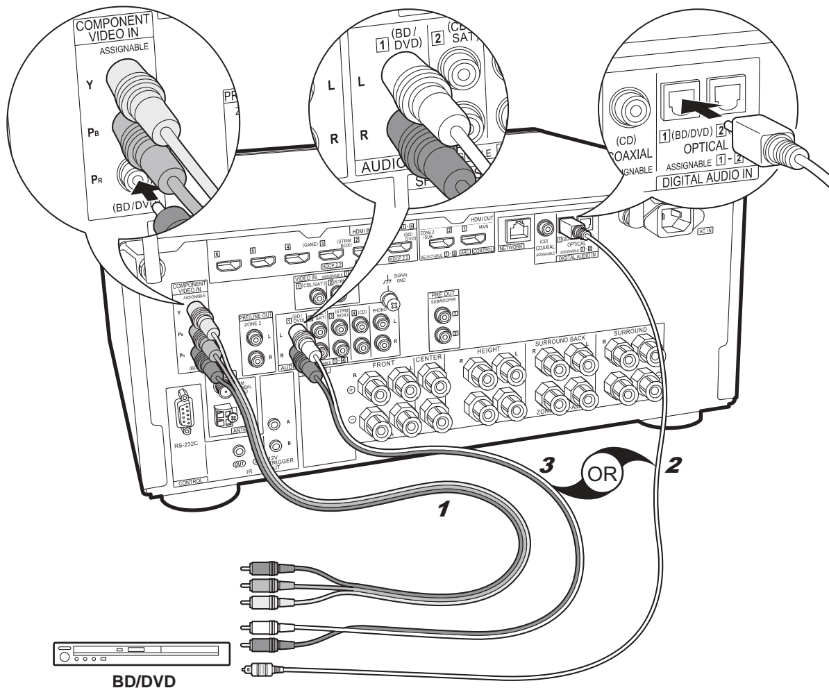
1 Component video cable, 2 Digital optical cable, 3 Analog audio cable
