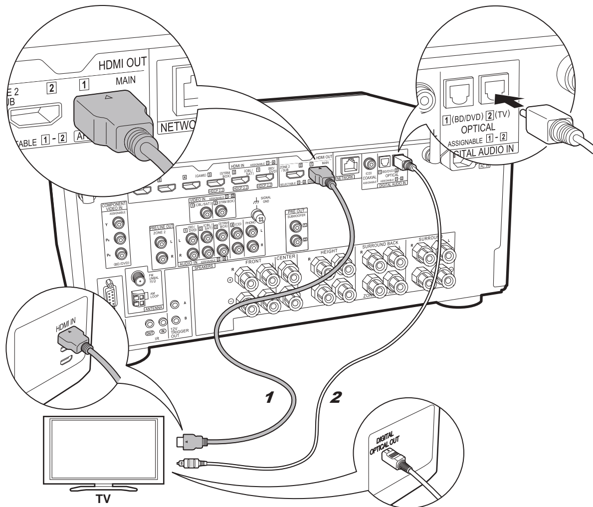
1 HDMI cable, 2 Digital optical cable
