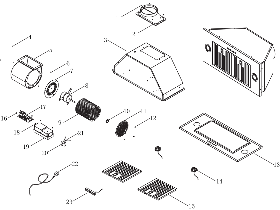
30" Range Hood
