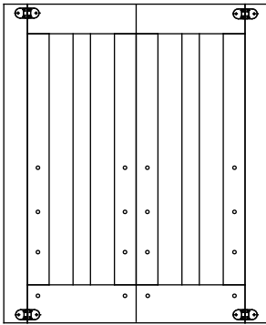
C Side panel (2) C. Panel lateral (2)
