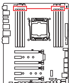
DIMM LEDs
