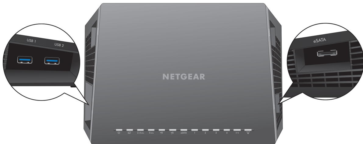
Figure 10. USB 3.0 and an eSATA port are located on the sides of the router
