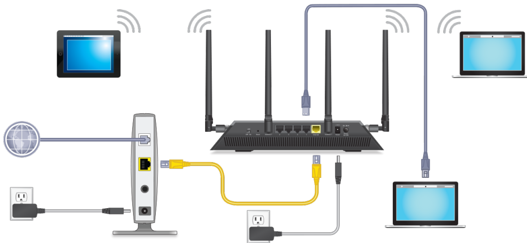
Figure 6. Router cabling
