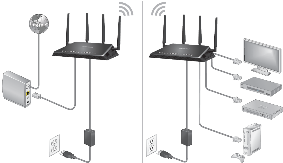
Figure 8. Router in bridge mode with an 802.11ac WiFi connection
