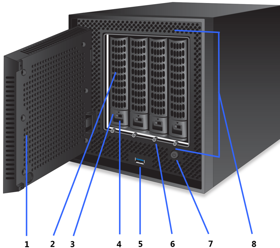
Figure 46. ReadyNAS 524X drive bays
