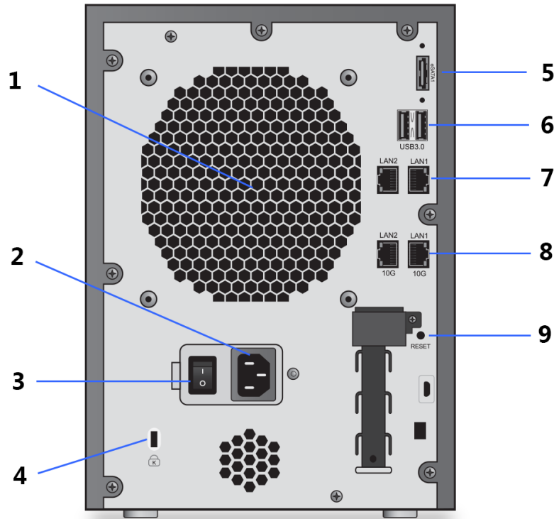
Figure 51. Rear panel ReadyNAS 626X
