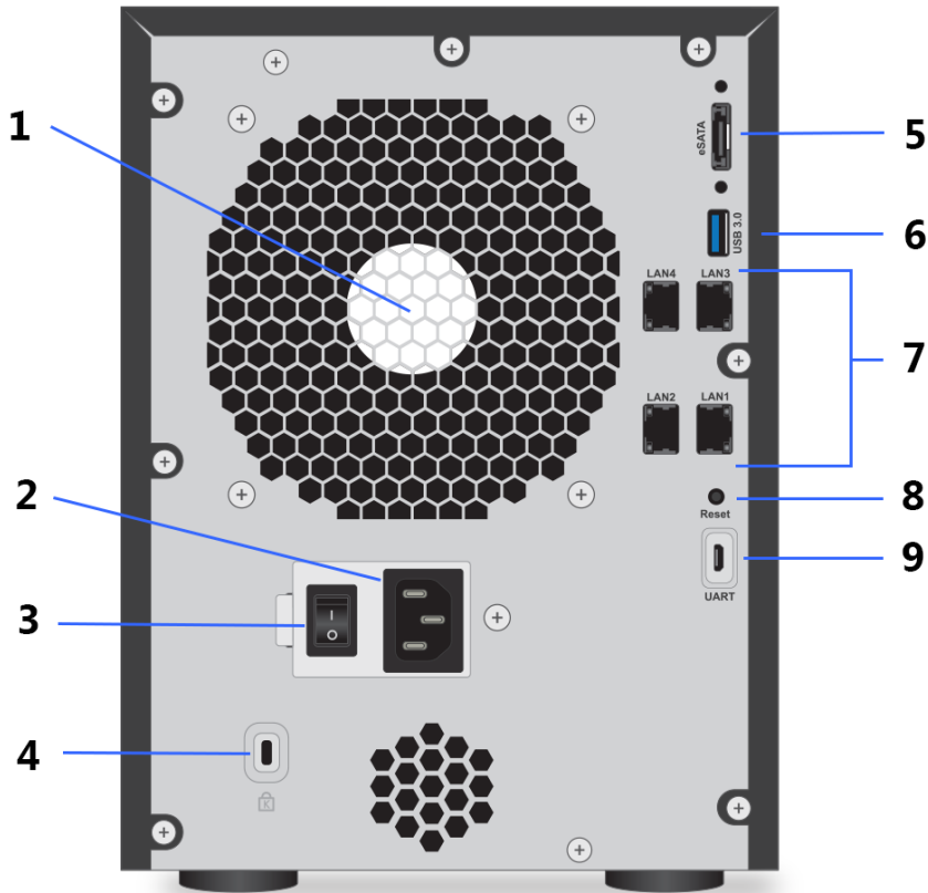
Figure 38. ReadyNAS 426 rear panel
