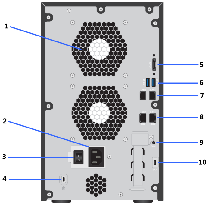
Figure 55. Rear panel ReadyNAS 628X
