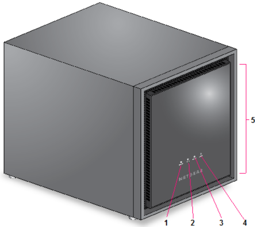
Figure 59. EDA 500 front and side panels
