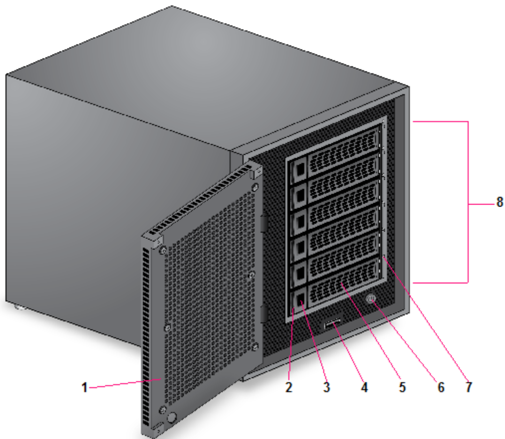
Figure 57. ReadyNAS 716X drive bays
