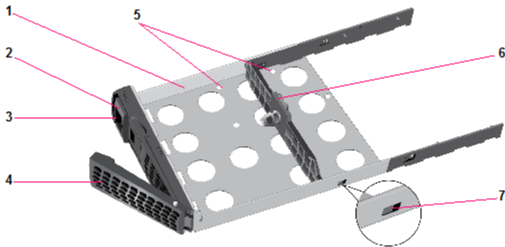
Figure 62. Standard disk tray
