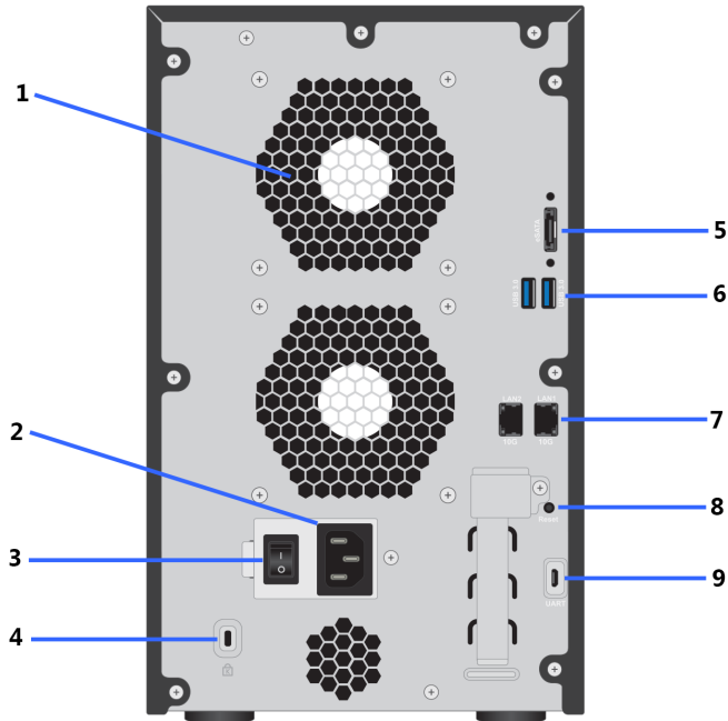
Figure 54. Rear panel ReadyNAS 528X
