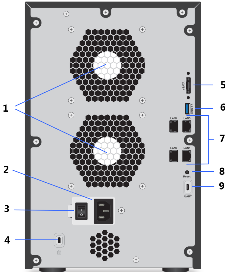
Figure 41. ReadyNAS 428 rear panel
