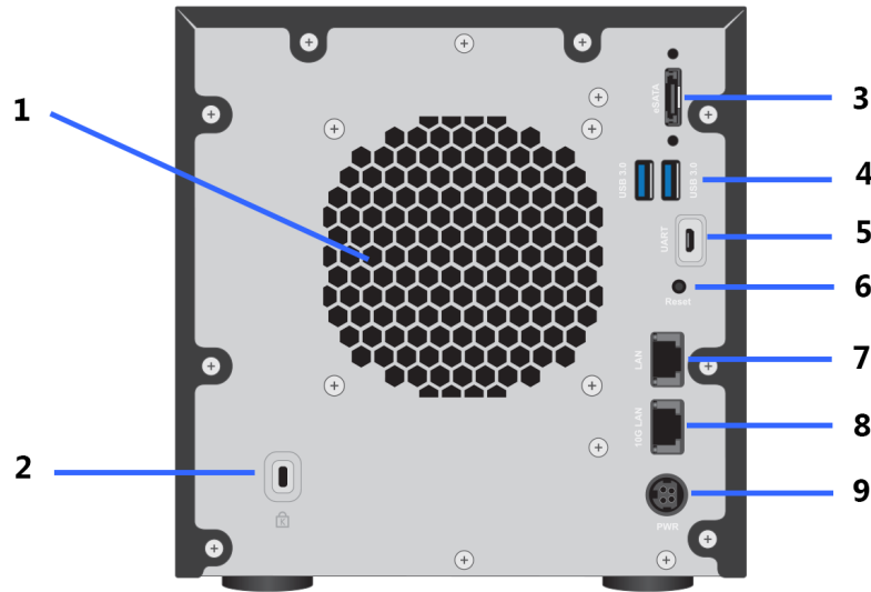
Figure 47. Rear panel ReadyNAS 524X
