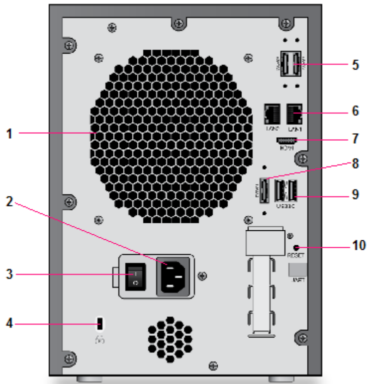
Figure 44. ReadyNAS 516 rear panel
