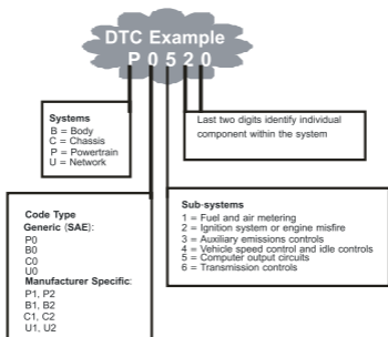
Figure 1-2: Explanation of a diagnostic trouble code.
