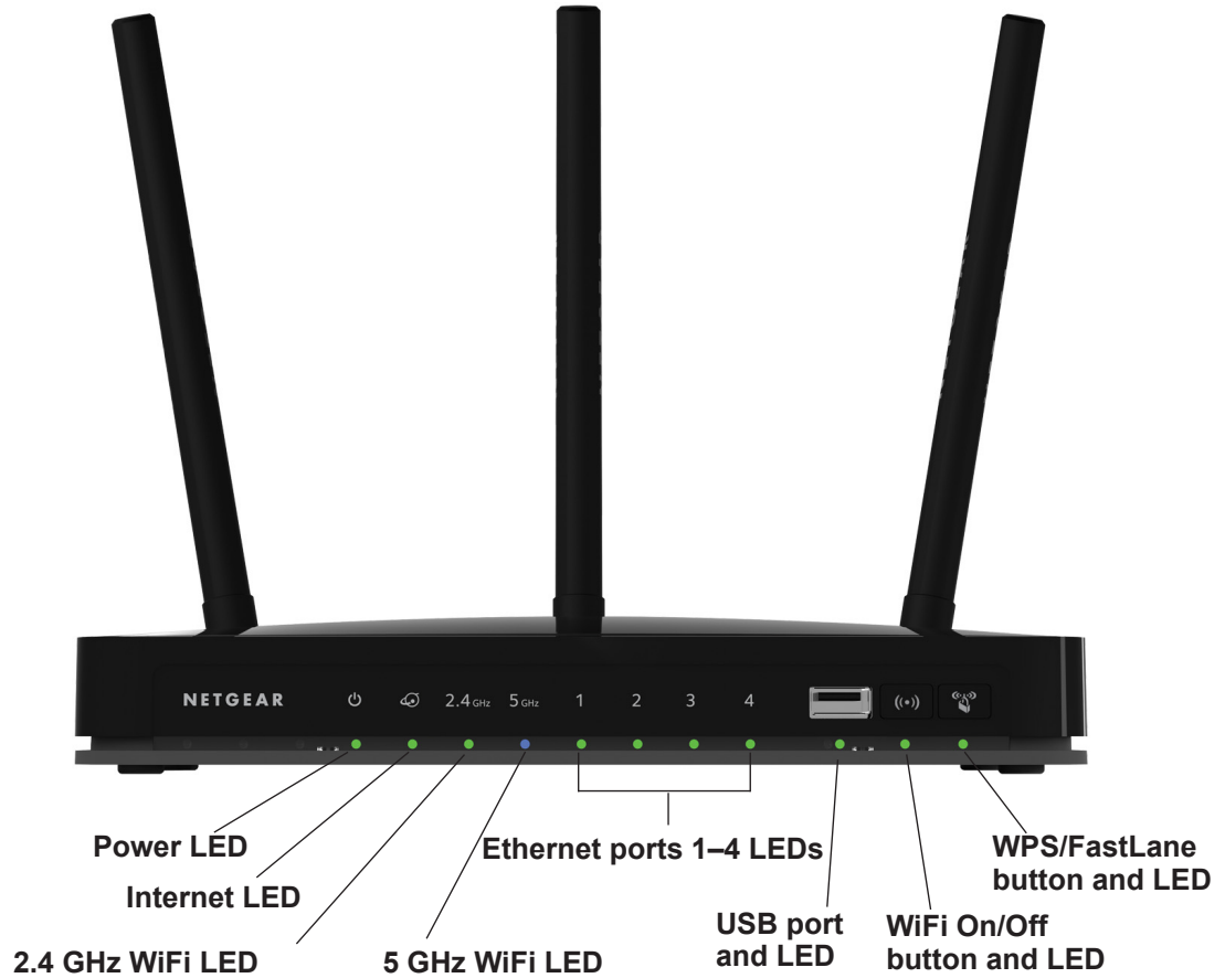
Figure 2. Front panel
