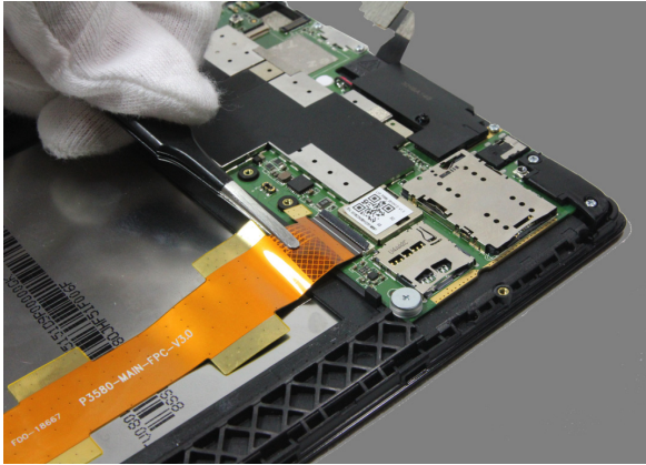
Figure 6-3. Pulling out the main FPC (from the main board side)
