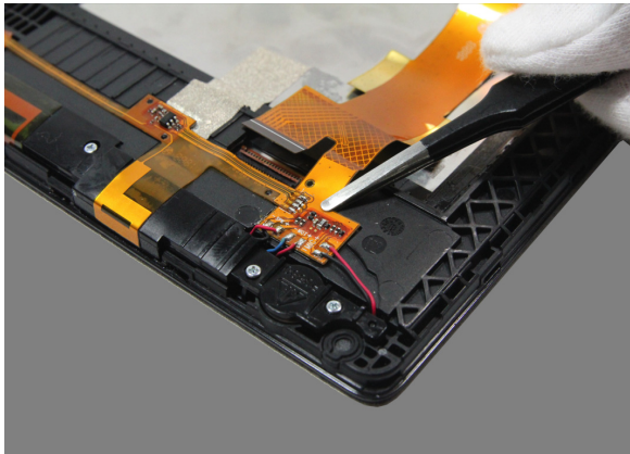
Figure 6-14. Detaching the main FPC
