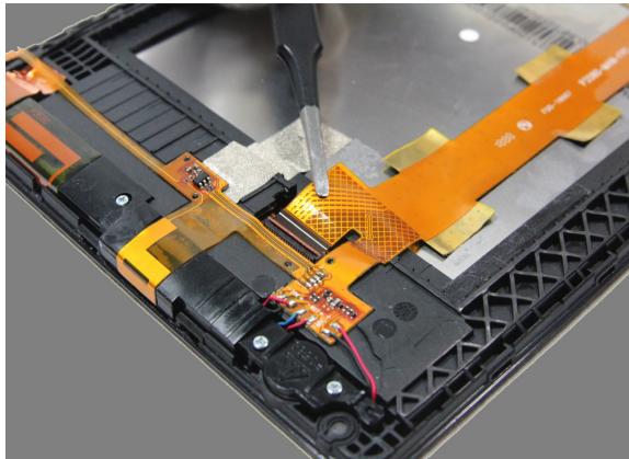
Figure 6-10. Pulling out the main FPC
