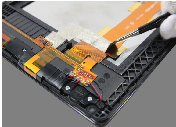
Figure 6-12. Removing the conductive fabric
