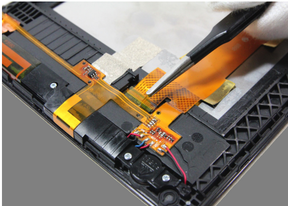
Figure 6-8. Removing the mylar on the connector of the main FPC
