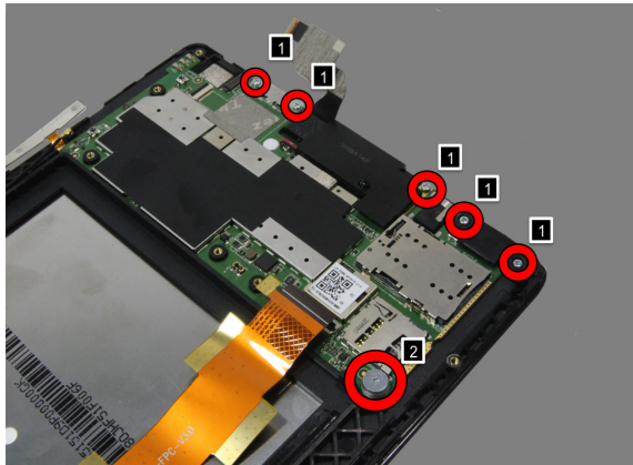
Figure 5-9. The screws on the bracket
