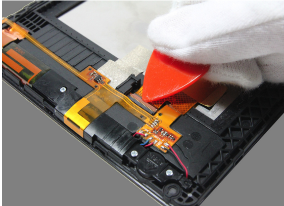
Figure 6-9. Unlocking the connector of the main FPC
