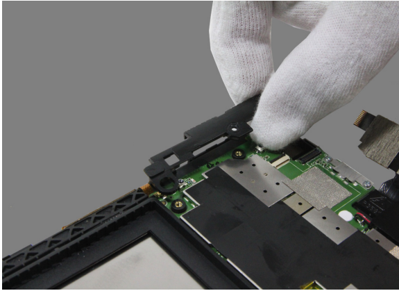
Figure 6-5. Removing the bracket
