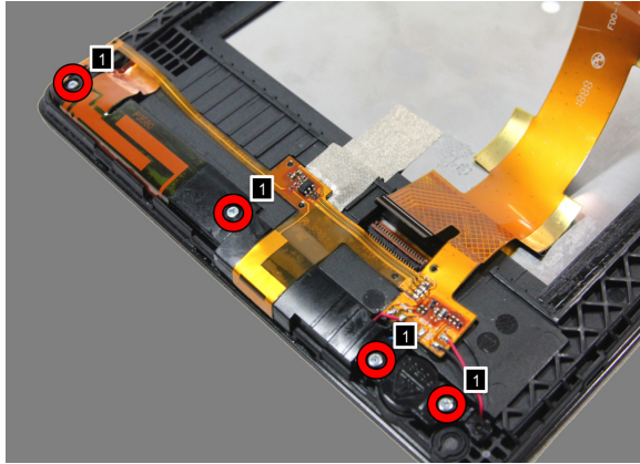
Figure 6-15. The screws on the bottom side speaker bracket
