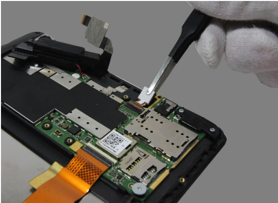
Figure 4-5. Pulling out the front camera FPC
