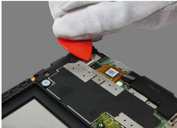
Figure 4-1. Unlocking the connector of the TP FPC
