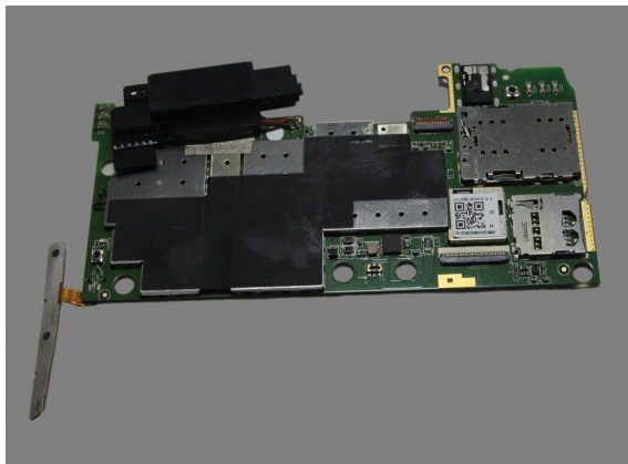
Figure 5-13. The removed the main board assembly
