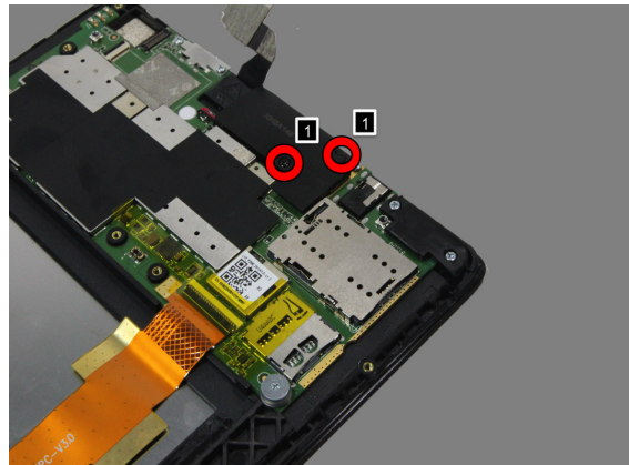
Figure 4-3. The screws on the top side speaker
