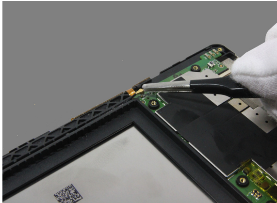
Figure 6-6. Detaching the LTE antenna cable
