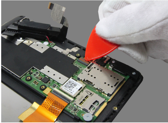
Figure 4-4. Unlocking the connector of the front camera FPC
