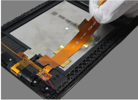
Figure 6-13. Detaching the main FPC
