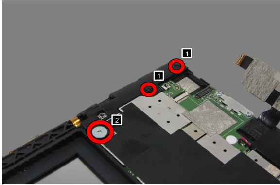
Figure 5-1. The screws on the bracket
