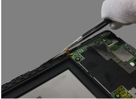
Figure 5-4. Detaching the side key FPC
