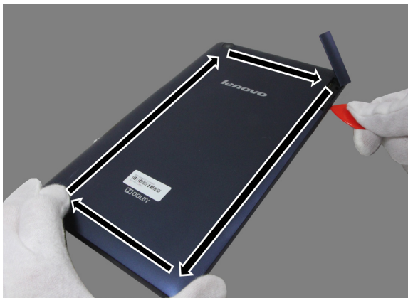
Figure 1-4. Unlocking the rear cover from the front module (along the joint line)
