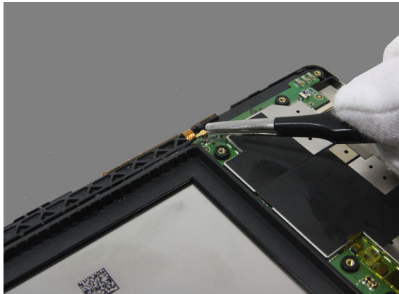
Figure 5-3. Detaching the antenna cable (Lenovo TAB 2 A8-50L/LC only)
