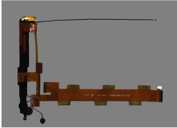
Figure 6-19. The removed the main FPC assembly (Lenovo TAB 2 A8-50L/LC)
