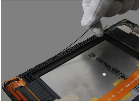
Figure 6-7. Detaching the LTE antenna cable
