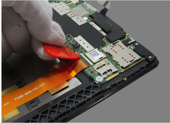
Figure 5-6. Unlocking the connector of the main FPC
