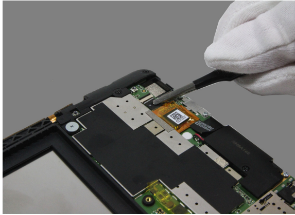
Figure 4-2. Pulling out the TP FPC
