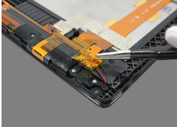
Figure 6-11. Removing the mylar
