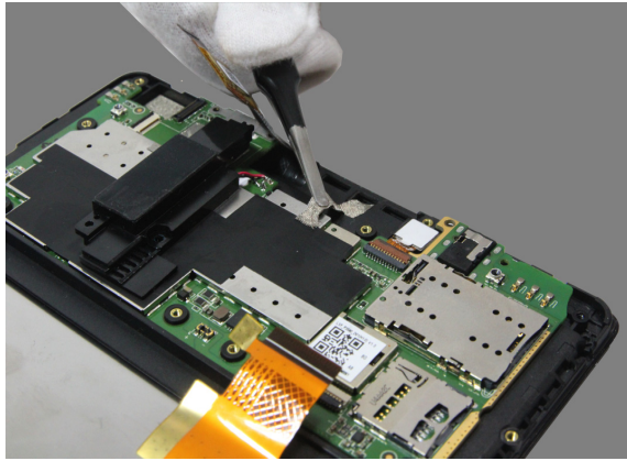
Figure 5-8. Removing the conductive fabric
