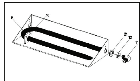
Figure 6. Burner bar connection
